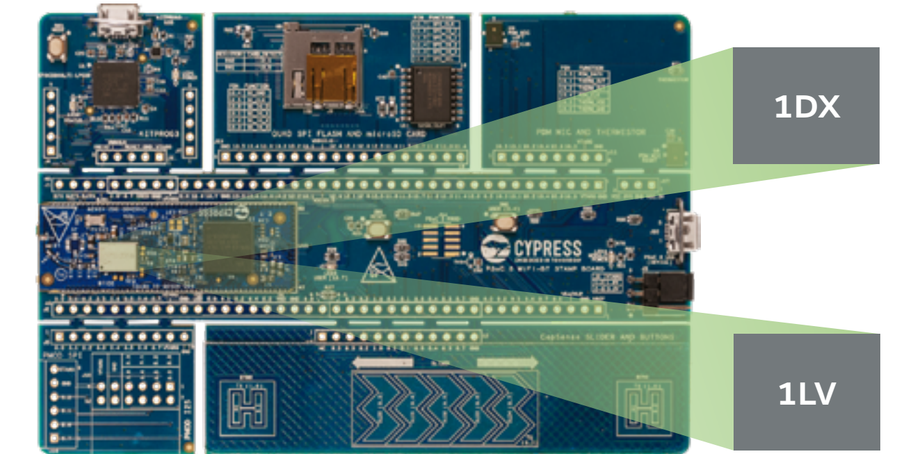
PSoC® 6 WiFi-BT Pioneer Kit
